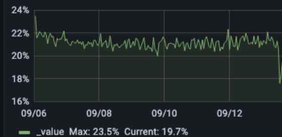
Memory Usage [%]
