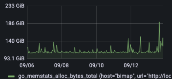
Memory Allocations
